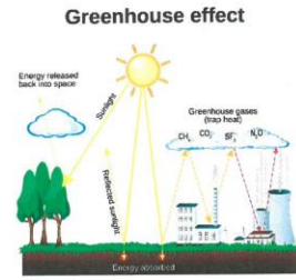
Figure 1-2 Greenhouse effect in remote Australia
