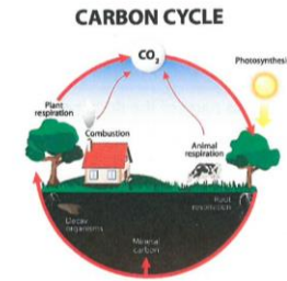
Figure 2-1 Carbon cycle in remote Australia
